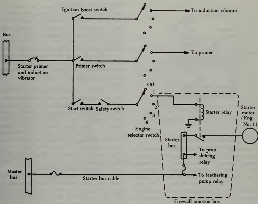
FIGURE 5-9. Starter control circuit.
